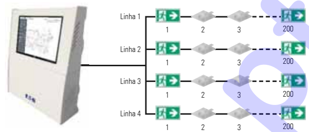
CGL+ Web Touchscreen Controller
